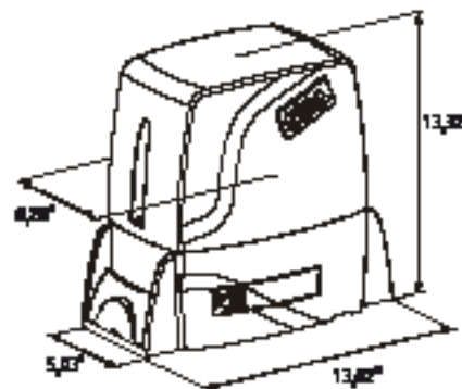
Dimensions (inches)
